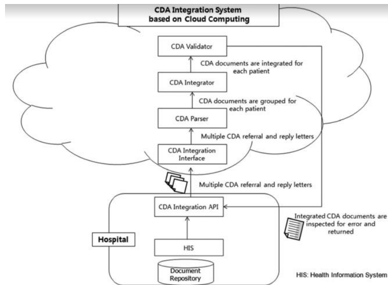
Fig 1: Proposed Approach
